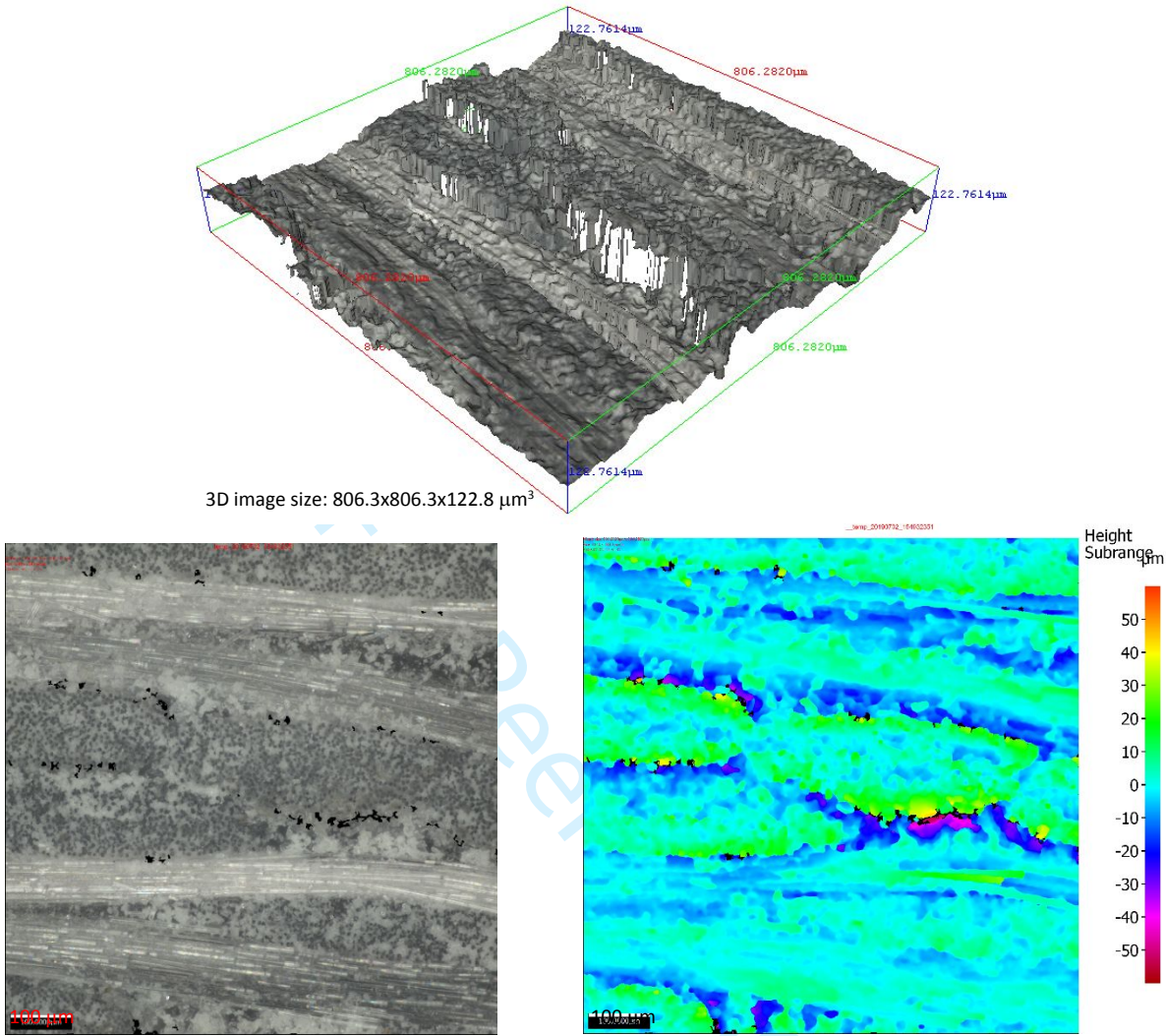
Figure 21. Surface texture of GFRP laminate after machining at 8000 rpm and 400 mm/min ( T = 178\text{ }^{\circ}\text{C} , S10z = 70.327\pm 9.155\text{ }\mu\text{m} ).
