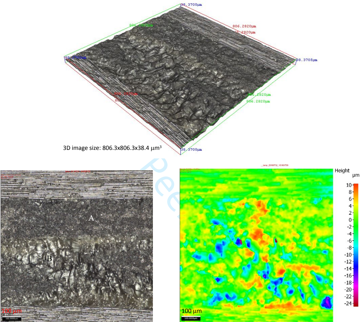
Figure 19. Surface texture of CFRP laminate after machining at 8000 rpm and 400 mm/min ( T = 218\text{ }^{\circ}\text{C} , S10z = 33.495\pm5.085\text{ }\mu\text{m} ).
