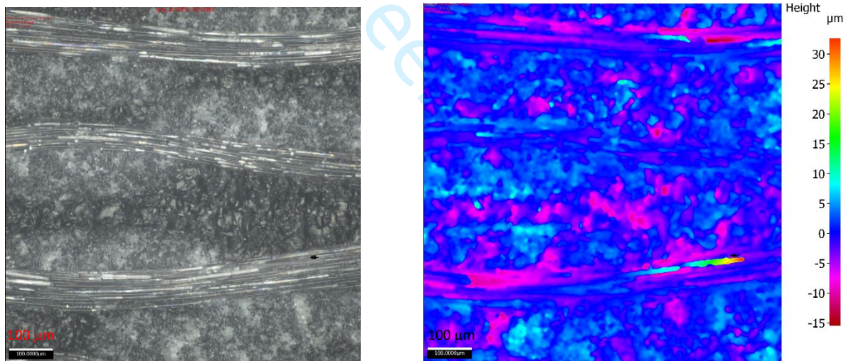
Figure 20. Surface texture of GFRP laminate after machining at 4000 rpm and 800 mm/min ( T = 120\text{ }^{\circ}\text{C} , S10z = 33.970 \pm 5.640\text{ }\mu\text{m} ).
