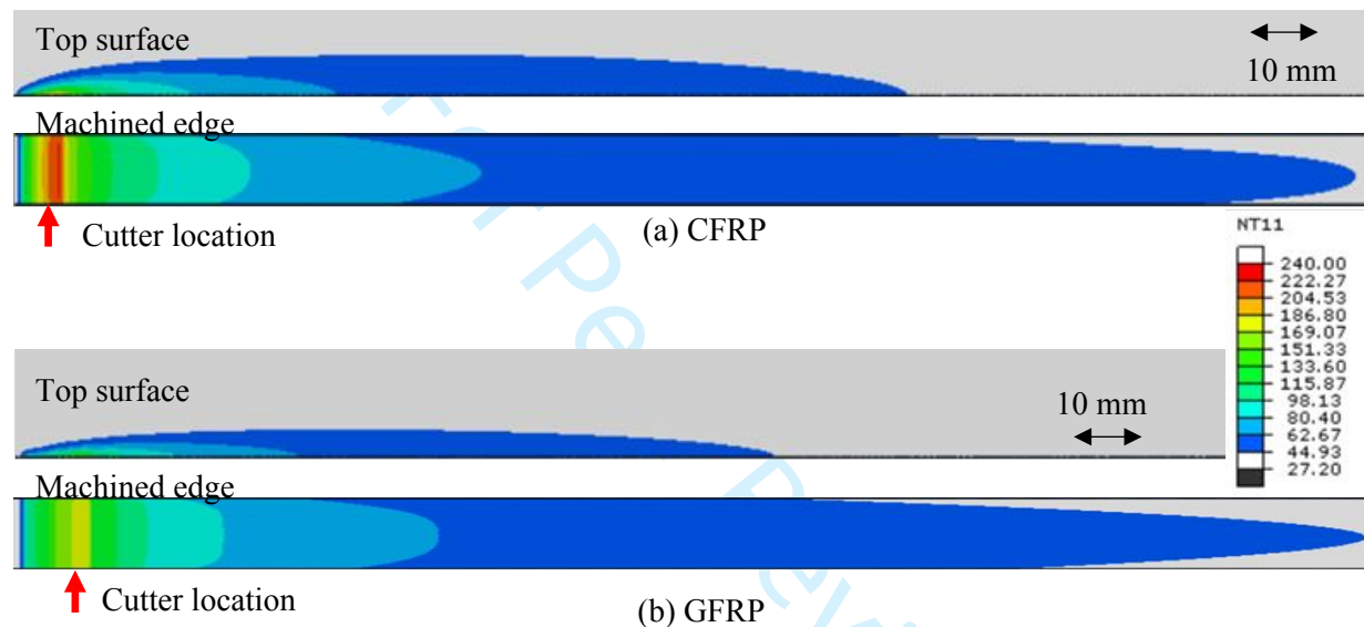
Figure 15. Contours of the temperatures in the machined workpiece for edge trimming at 8000 rpm and 400 mm/min, (a) CFRP and (b) GFRP.
