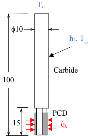
Figure 4. Numerical model for the cutter.
