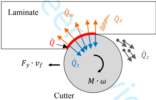
Figure 1. Heat partition is edge trimming operation.
