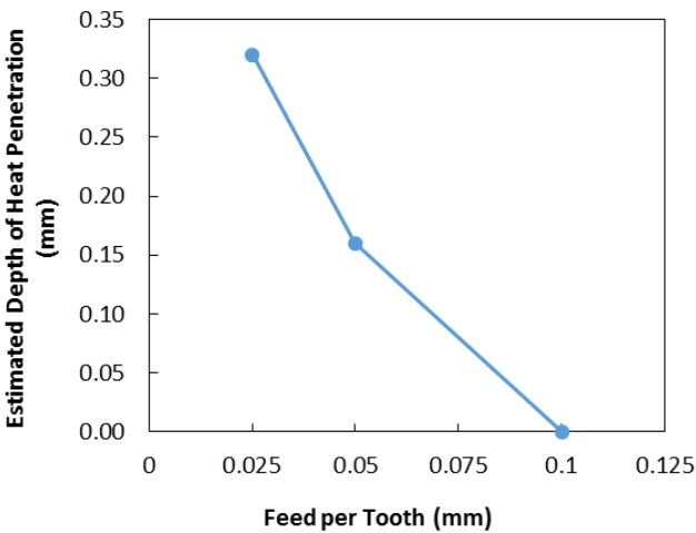
Figure 17. Estimated depth of thermal damage for the CFRP at different cutting conditions.
