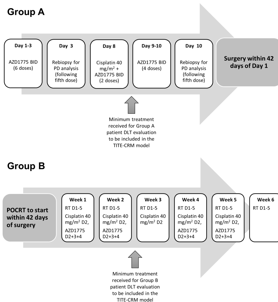
Figure 1 Wisteria trial schema. Group A patients were required to have received a minimum treatment of chemotherapy (cisplatin) and AZD1175 in combination to be DLT evaluable. Group B patients were required to have received a minimum of 2 weeks of treatment (half the total scheduled AZD1775 dose) to be DLT evaluable. DLT, dose-limiting toxicity; PD, pharmacodynamic; TITE-CRM, time-to-event continual reassessment method.
