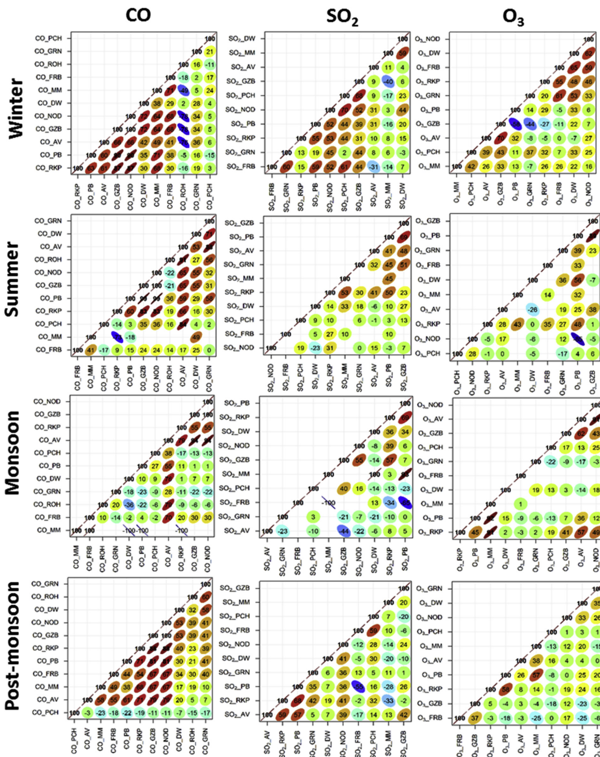
Fig. 6. Correlation matrix showing the relationships between CO, SO 2 and O 3 over the period at all sites. The plot shows the Pearson correlation coefficients expressed as -100 to 100. 100 is perfect correlation, zero is no correlation and -100 is a perfect inverse correlation.
