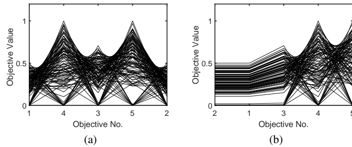
Fig. 3. The solutions of the SPEA2+SDE for DTLZ5(3,5) with different order of objectives. The results before and after the rearranging of the order of objectives are shown at left and right, respectively.
