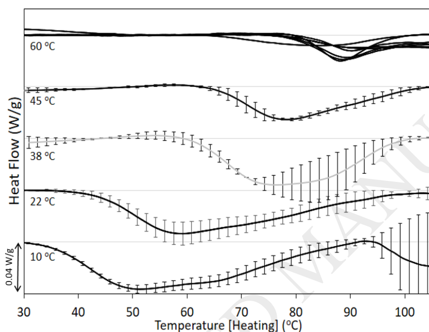
Figure 4. Melting DSC endotherm of 40% maltodextrin gels set for four days at the indicated temperature. A heating rate of 5^{\circ}\text{C}/\text{min} was utilized with a reference cell of water. Error bars represent the standard deviation of three replicates.
