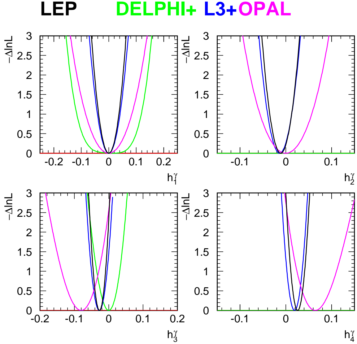
Figure 6.2: The \log \mathcal{L} curves of DELPHI, L3, and OPAL experiments and the LEP combined curve for the four neutral TGCs h_i^\gamma , i = 1, 2, 3, 4 . In each case, the minimal value is subtracted. Note, DELPHI did not interpret its measurements in terms of neutral gauge couplings of dimension 8 operators, hence does not enter in the combination for h_{2/4}^V .
