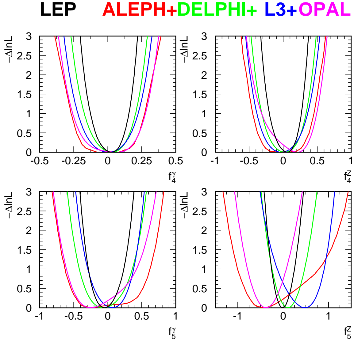
Figure 6.4: The \log \mathcal{L} curves of the four experiments, and the LEP combined curve for the four neutral TGCs f_i^V , V = \gamma, Z , i = 4, 5 . In each case, the minimal value is subtracted.
