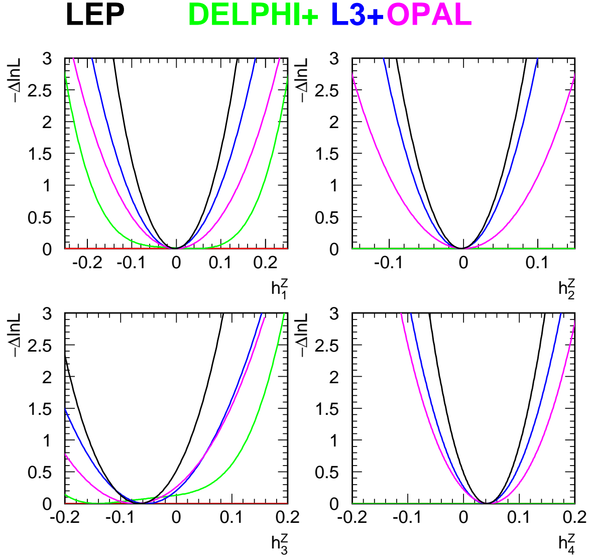
Figure 6.3: The \log \mathcal{L} curves of the DELPHI, L3, OPAL experiments and the LEP combined curve for the four neutral TGCs h_i^Z , i = 1, 2, 3, 4 . In each case, the minimal value is subtracted. Note, DELPHI did not interpret its measurements in terms of neutral gauge couplings of dimension 8 operators, hence does not enter in the combination for h_{2/4}^V .
