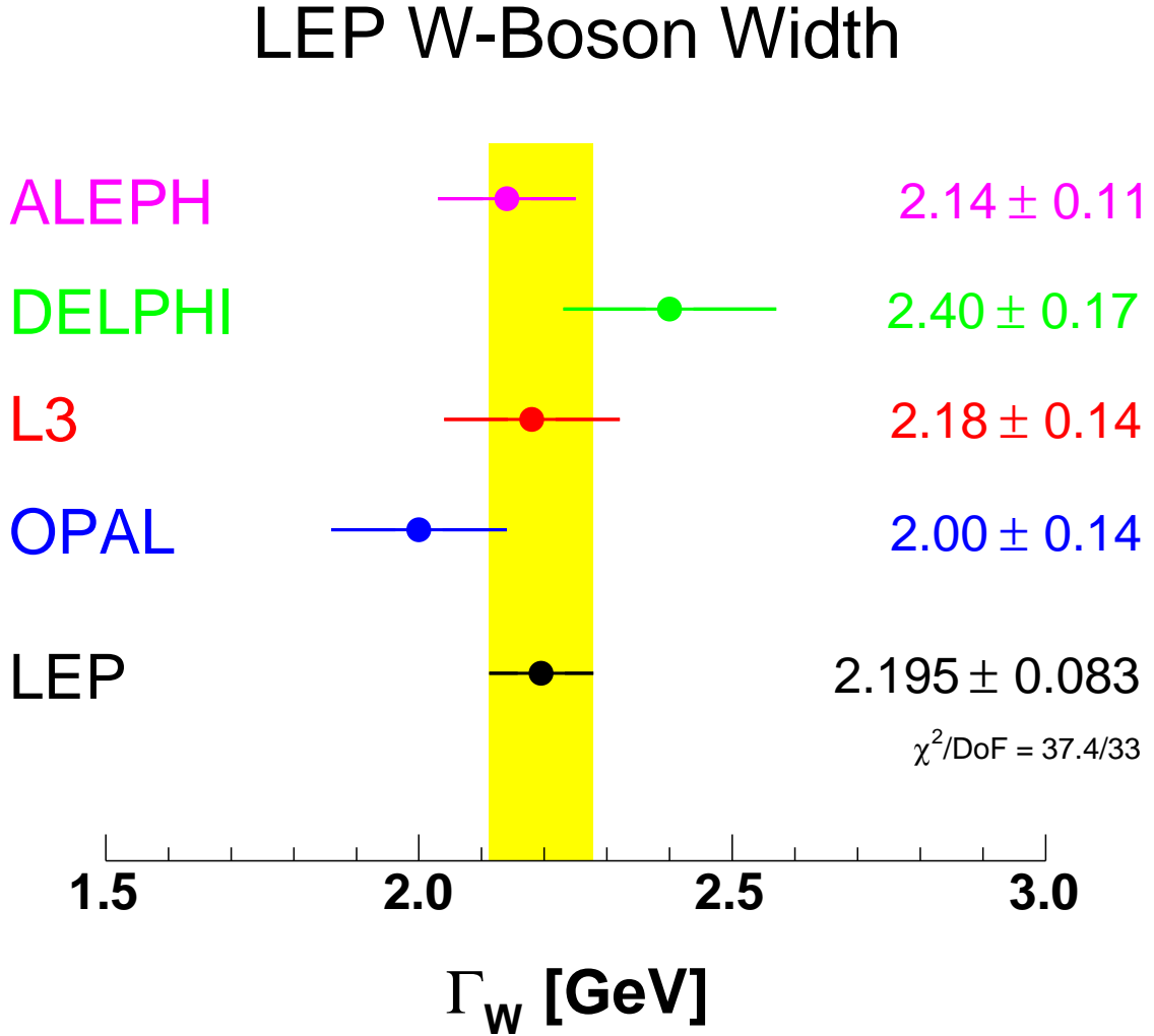
Figure 7.3: The measurements of the W-boson width obtained by the four LEP collaborations (as published) together with the LEP combined result. The combined value includes correlations between experiments, between different energy points, and between the q\bar{q}\ell\nu_\ell and q\bar{q}q\bar{q} channels. A revised estimation of systematic uncertainties due to colour reconnection and Bose-Einstein correlations is applied to the input of the individual measurements to the LEP combined results in order to take the direct determination of FSI parameters into account.
