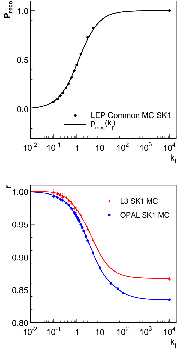
Figure 4.1: Top: Reconnection probability as a function of the SK1 model parameter, k_I , together with an approximate curve p_{\text{reco}}(k_I) to guide the eye. Bottom: Monte-Carlo calculation and parametrisation of the particle-flow ratio, r(k_I) , for L3 and OPAL, shown as triangles and circles, respectively.
