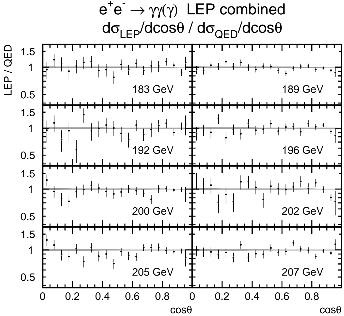
Figure 2.2: Combined differential cross-sections relative to the QED expectation. The error bars shown include the statistical and systematic experimental errors. The theory uncertainty is small, decreasing from 1.0% to 0.5% for increasing |\cos\theta| .
