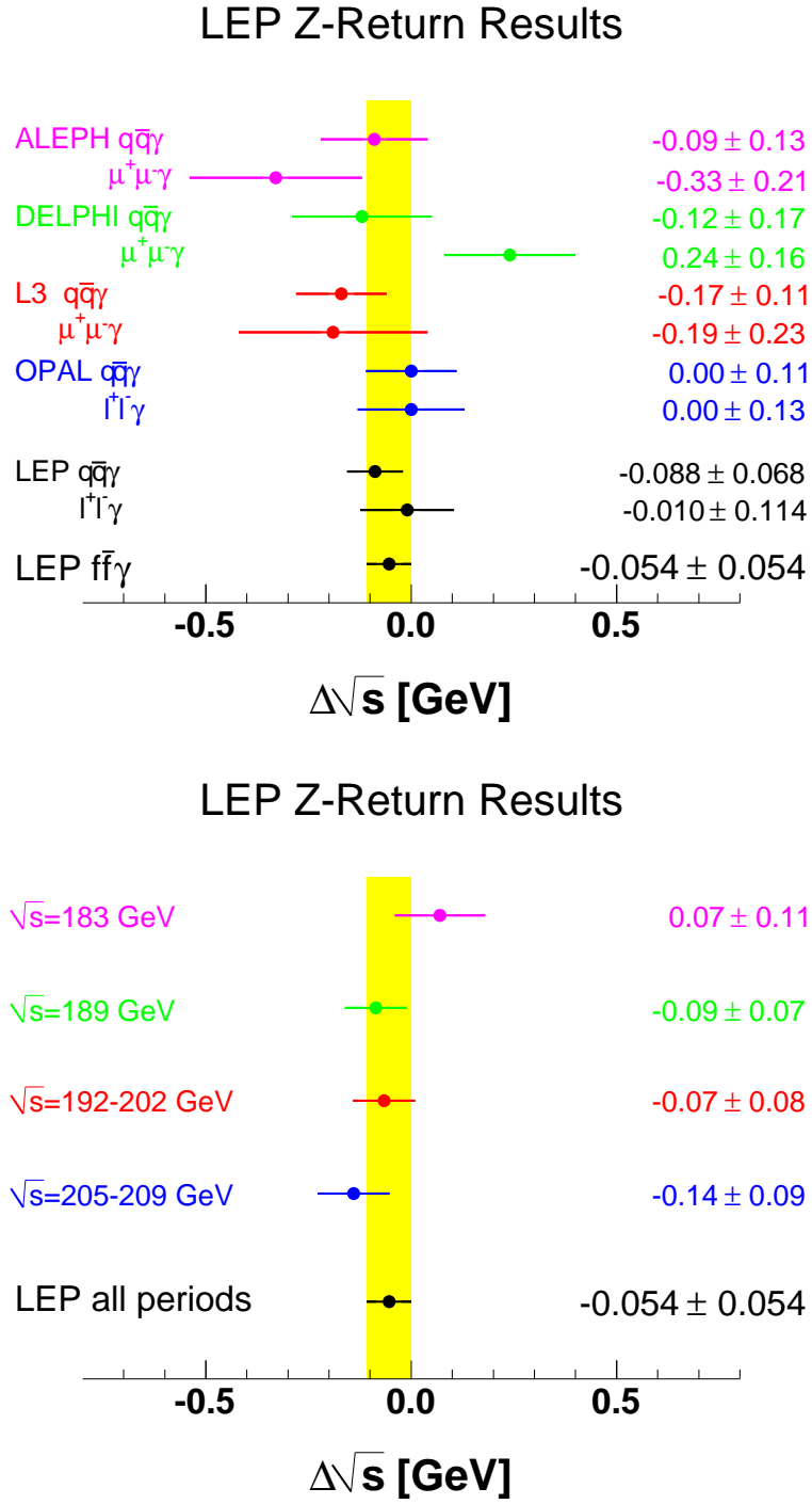
Figure C.2: Difference between the energy determined in Z-return events and the nominal LEP centre-of-mass energy, \Delta\sqrt{s} , for the different experiments and final states (top), and for the data taking periods with energies well above the W-pair threshold (bottom). The individual measurements as well as the LEP combined values take systematic uncertainties and their correlations into account.
