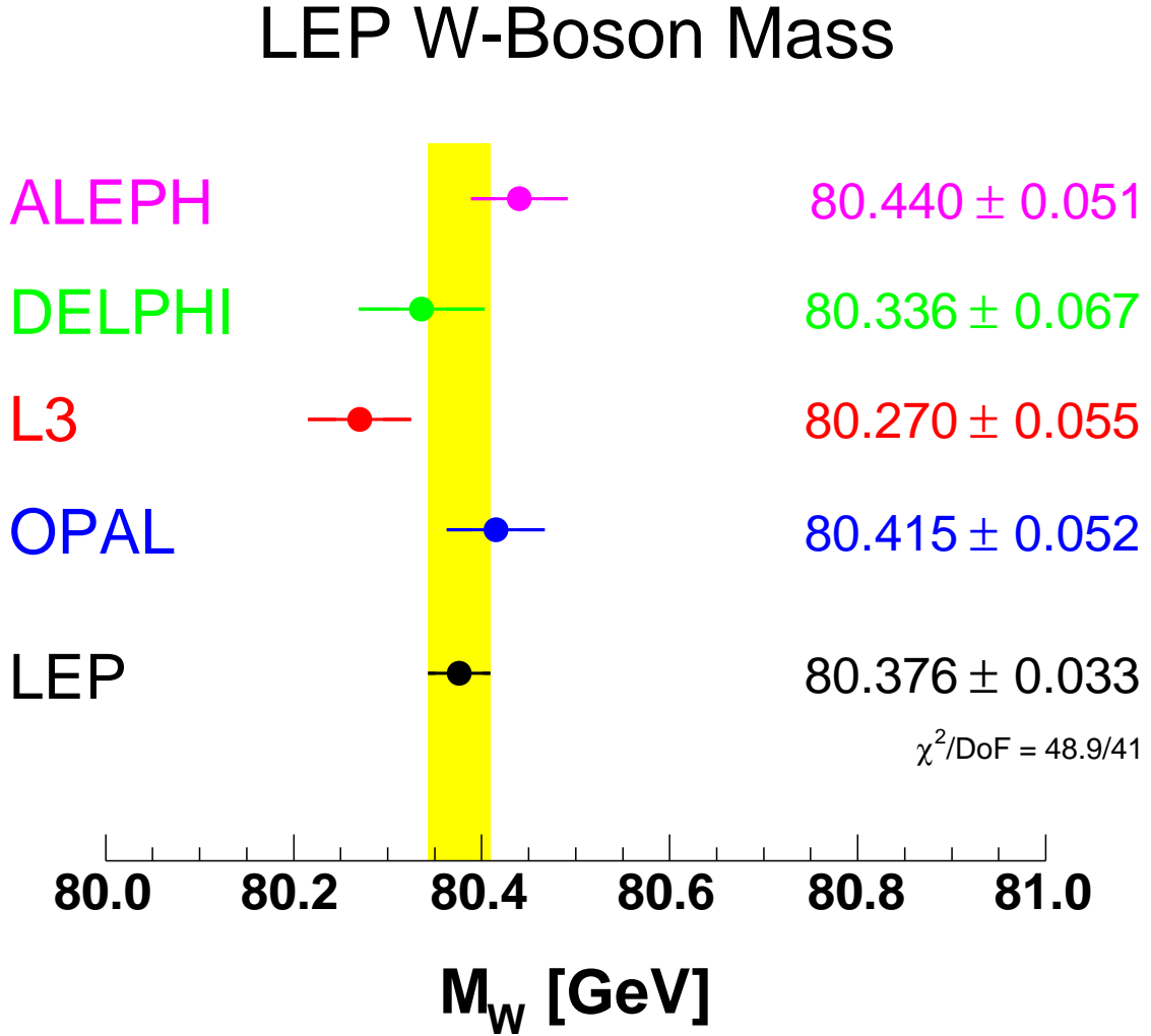
Figure 7.1: The measurements of the W-boson mass obtained by the four LEP collaborations (as published) together with the LEP combined result. The combined value includes correlations between experiments, between different energy points, and between the q\bar{q}\ell\nu_\ell and q\bar{q}q\bar{q} channels. A revised estimation of systematic uncertainties due to colour reconnection and Bose-Einstein correlations is applied to the input of the individual measurements to the LEP combined results in order to take the direct determination of FSI parameters into account.
