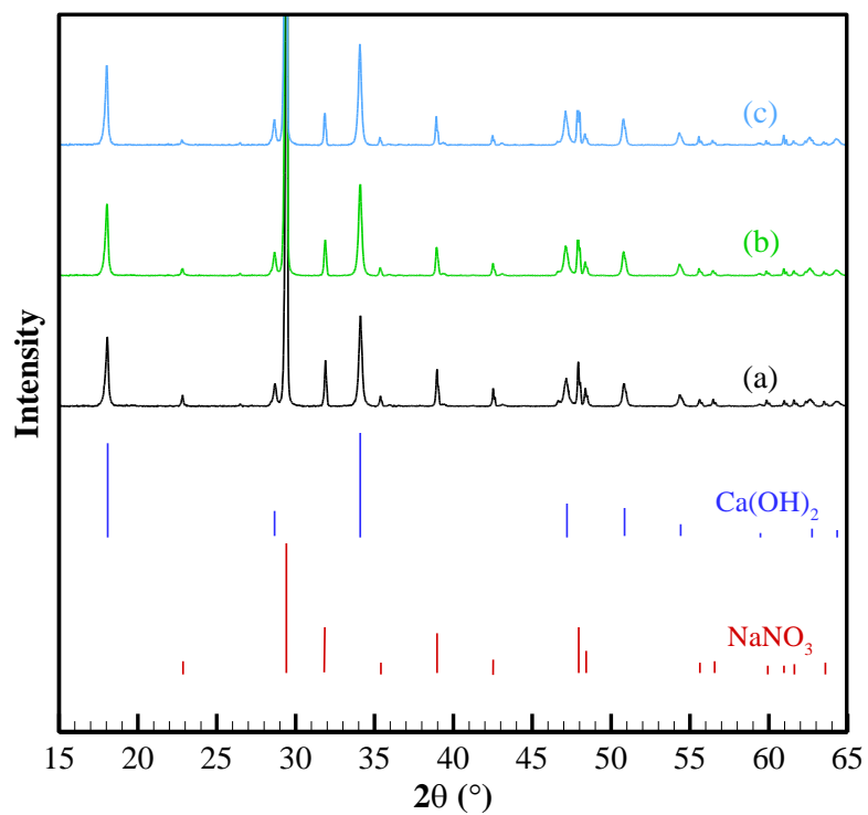
Fig. 6 XRD patterns of \text{NaNO}_3/\text{Ca}(\text{OH})_2 composite: (a) before thermal cycling; (b) after 100 thermal cycles; (c) after 200 thermal cycles.
