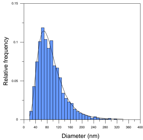
Figure 2. Nanoparticle size distribution measured by SEM
