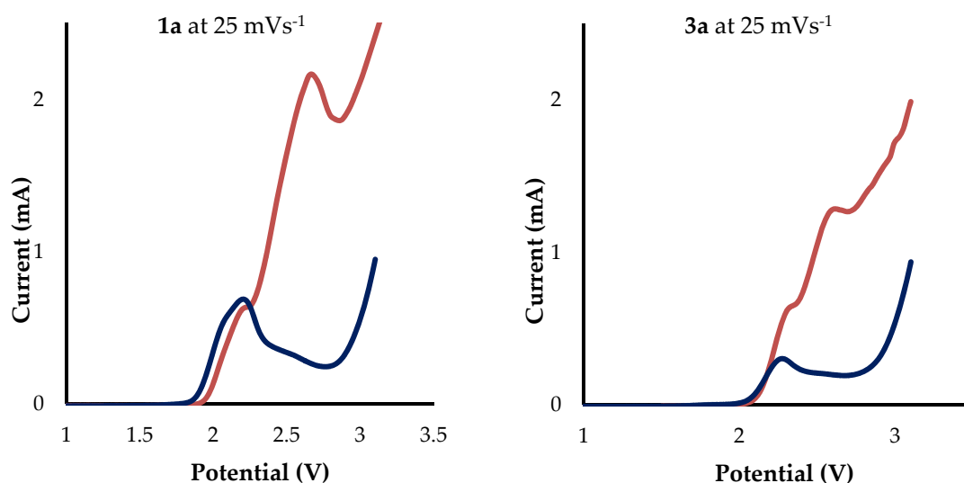
Figure 3. Linear sweep voltammetric oxidative response from surveying the scan rate of 1a and 3a . Conditions: MeCN/MeOH or H 2 O (10:1), 500 mM Bu 4 NClO 4 , 22.0 mM of analyte, W.E. = GC, C.E. = Pt wire, R.E. = Ag + /Ag (-0.057 V versus Fc + /Fc), \nu = 5-250 mVs -1 . Data for \nu = 25 mVs -1 shown for clarity.† Solvent system: Red = MeCN/MeOH, Blue = MeCN/H 2 O.
