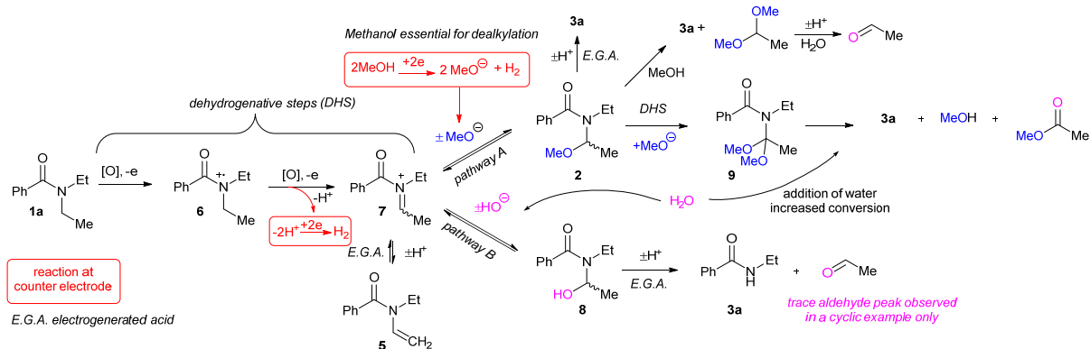
Scheme 2 Possible reaction mechanisms for the formation of 3a .
