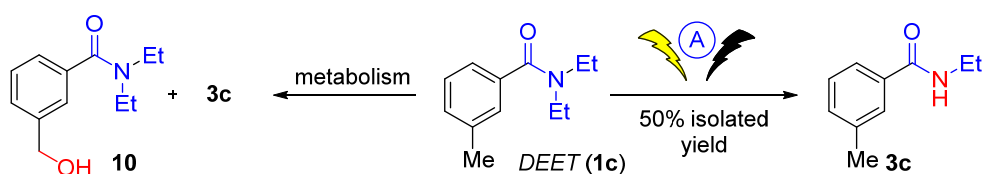
Scheme 3. Application of the methodology to the tractable preparation of the human metabolites of an insect repellent (DEET).
