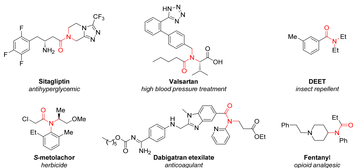
Figure 1. Examples of pharmaceuticals and agrochemicals that contain a tertiary amide
