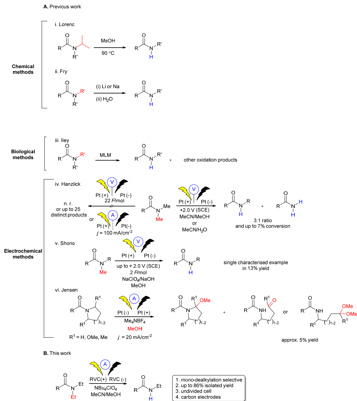
Scheme 1. Previous methods to N -dealkylation of tertiary amides and the new route disclosed.
