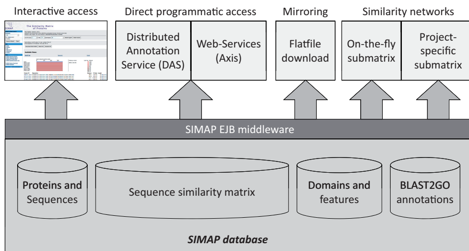
Figure 1. Schematic representation of the SIMAP database contents and access facilities.
