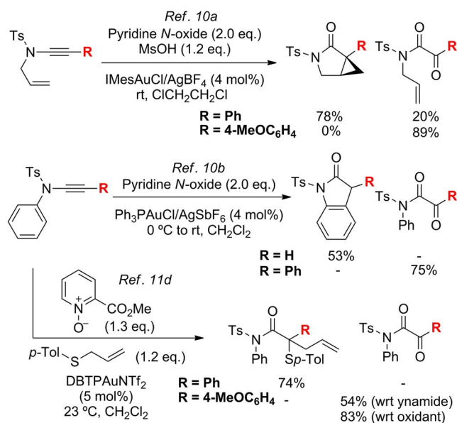
Scheme 2. Gold-catalysed oxidative reactions: The impact of ynamide C-substitution on \alpha -ketoimide formation versus desirable inter- or intramolecular pathways. DTBP = tris(2,4-di- t -butylphenyl)phosphite.
