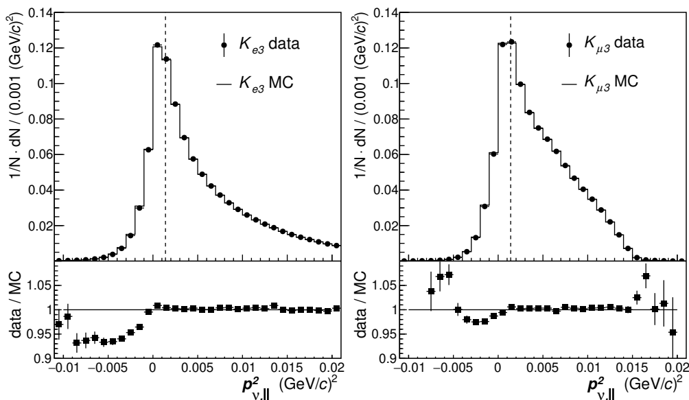
Figure 4. Normalized p_{\nu,\parallel}^2 distributions of data and MC simulated samples for K_{e3}^{\pm} (left) and K_{\mu3}^{\pm} (right) modes and corresponding Data/MC ratios. The simulated samples include signal and backgrounds. The vertical dashed lines indicate the p_{\nu,\parallel}^2 > 0.0014 \text{ (GeV/c)}^2 cut applied.
