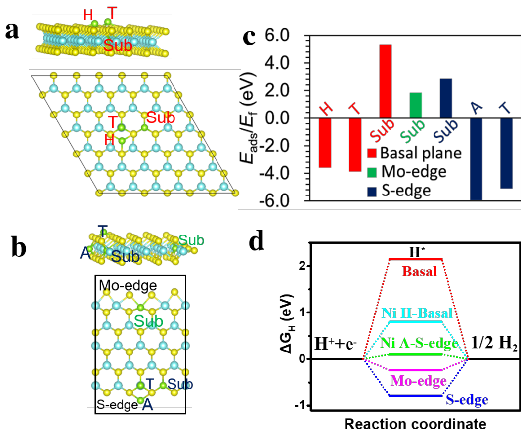
Figure 7 (a) Atomistic configuration of Ni adsorbed at the top of the Mo sites (T) and the center of the hexagon sites (H) on the basal plane and substitution of Mo atom with Ni in monolayer MoS 2 . (b) Atomistic configuration of Ni adsorbed at T and A sites at the S-edge and substitution of Mo atom with Ni at the Mo-edge and S-edge. (c) Adsorption energy of Ni on MoS 2 and formation energy of substitution of Mo atom with Ni atom in MoS 2 . (d) Gibbs free energies for H* adsorbed at basal plane, Mo edge and S edge with and without Ni adsorption/substitution.
