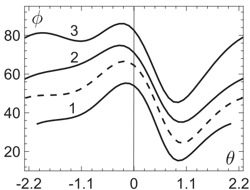
FIG. 7. The dependence of the contact angle \phi formed by the free surface and the side wall of the disk on the azimuthal (polar) angle \theta in the plane of the disk parameterizing the disk's rim in the representative sector. The jet's centerline corresponds to \theta = 0 . The base case is shown as the dashed line, and curves 1, 2, and 3, as in Fig. 6, correspond to \Omega = 240 \text{ rad s}^{-1} , Q = 10 \text{ ml s}^{-1} , and z_{cl} = 0.5 \text{ mm} , respectively.
