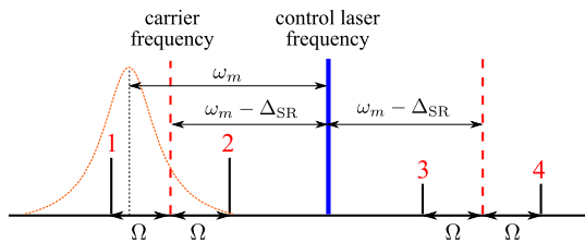
FIG. 6. A schematic showing the relevant four sidebands and their frequencies with respect to the carrier frequency \omega_0 and control laser frequency \omega_0 + \omega_m - \Delta_{\text{SR}} ( \Delta_{\text{SR}} is the signal recycling detuning frequency of the interferometer). The control laser is detuned away from the optomechanical cavity resonant frequency by \omega_m ; the resonance profile of the cavity is illustrated by the Lorentzian shape.
