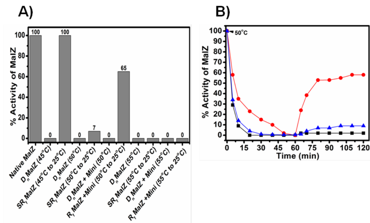
Fig. S5. Reactivation of thermally inactivated MalZ. A) 0.5μM MalZ was subjected to thermal denaturation at three different temperatures (as shown in different bars) in the absence or presence of 2.5 μM minichaperone until its activity was reduced to zero. Samples were then cooled down to 25° C and reactivation of MalZ was measured. The extent of regain of activity is expressed as a percentage of the activity of the same amount of native MalZ. Here D n , SR f and R f represents denatured, spontaneously refolded and refolded MalZ respectively. B) Time course of reactivation of MalZ at 25°C in the absence or presence of lysozyme and minichaperone. In this experiment, MalZ was denatured at 50°C (indicated by arrow) for 60 min in the absence (■) or presence of 2.5 μM lysozyme (▲) or 2.5μM minichaperone (●, Red color). After 60 min, samples were then cooled to 25°C and reactivation of MalZ was measured over time.
