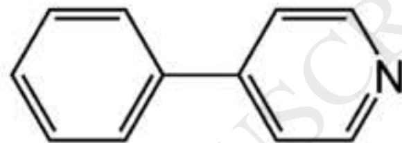
4-Phenylpyridine
