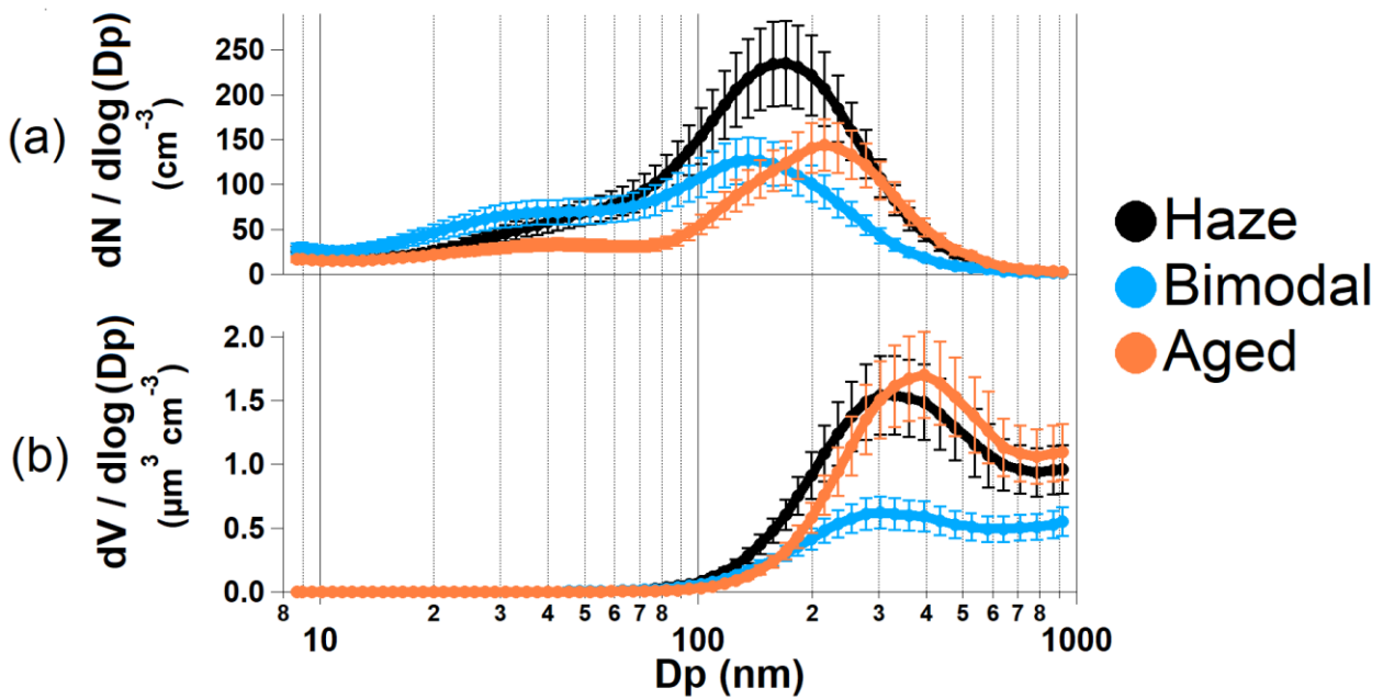
341 Fig. 2. Aerosol (a) number and (b) volume size distributions for the three accumulation 342 categories. 343 344
