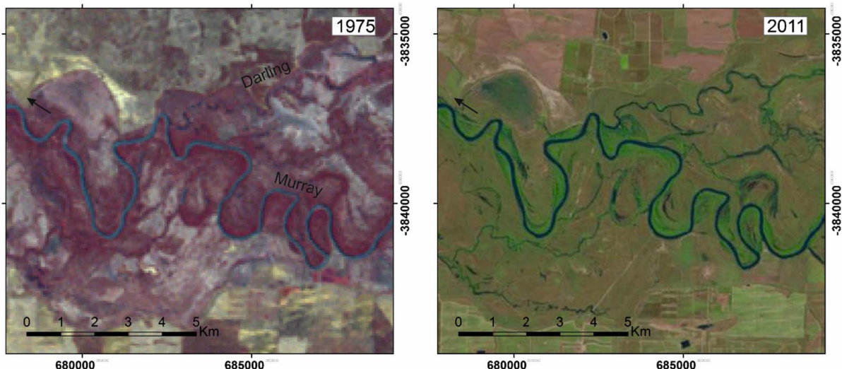
Fig. 13. Landsat images showing the confluence of the Murray and Darling rivers in Australia. The images show abandoned meander loops in the floodplain surface suggesting historic channel mobility, but over the 36-year image sequence there is no evidence of active meandering and the confluence position remains fixed.
