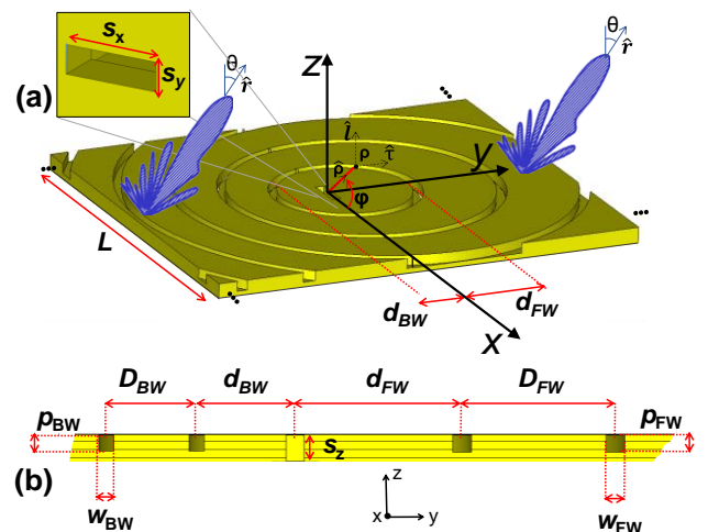
Fig.1 Geometry of analyzed structure. (a) 3D view. (b) Cross-sectional view in the plane z - y .
