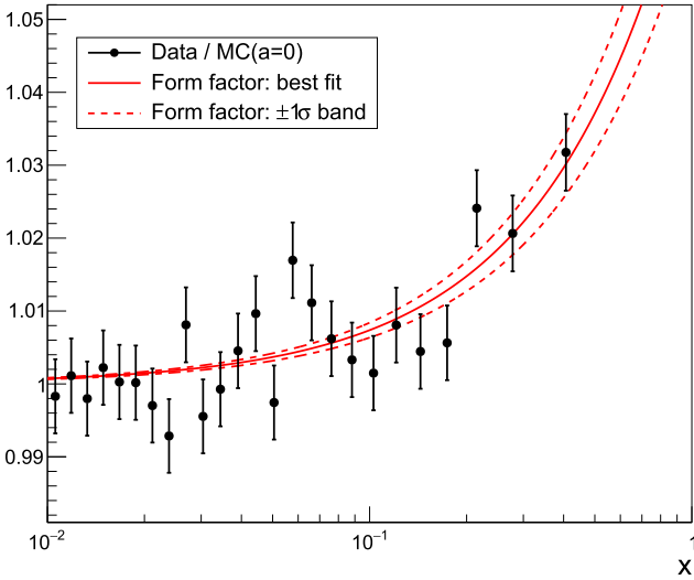
Fig. 3. Ratio of the reconstructed x distributions for data and MC, where the MC sample corresponds to a = 0 . The effect of a positive TFF slope ( a > 0 ) is clearly seen in this illustration. Data and MC events are distributed into 25 equally populated bins; the horizontal positions of the markers correspond to the bin barycentres. The solid line represents |\mathcal{F}(x)|^2 with the measured central slope value: a = 3.68 \times 10^{-2} . The dashed lines indicate the \pm 1\sigma band. Only the statistical uncertainties are shown.
