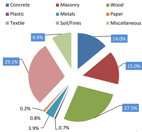
Figure 3 - Composition of CDW (adapted from Schlauder and Brickner (1993))
