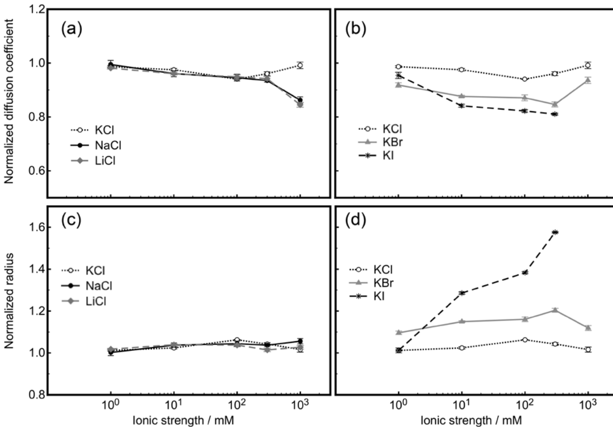
Figure 2: (a, b) Diffusion coefficients and (c, d) radii of PMPC chains, normalized to those in pure water (diffusion coefficient 32.0 \mu\text{m}^2 \text{s}^{-1} with corresponding radius 2.7 nm), as a function of ionic strength, where either the cations (a, c) or the anions (b, d) is varied.
