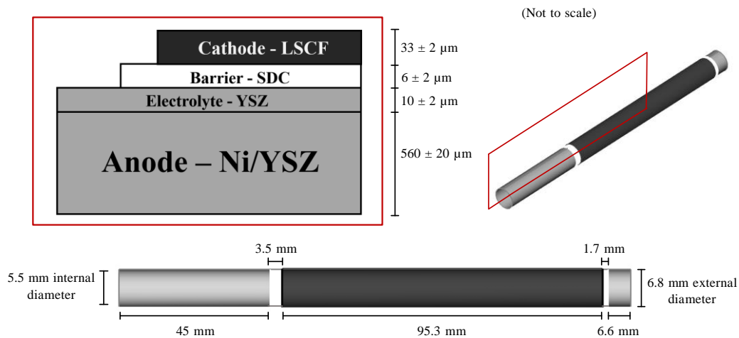
Figure 1: Tubular SOFC configuration.
