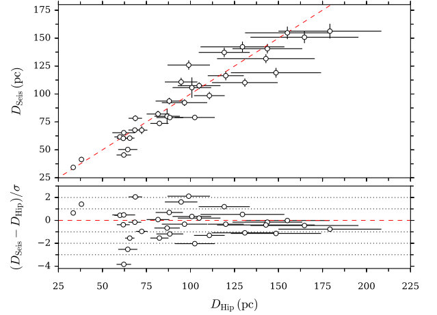
Figure 9. Top: Comparison between distances from seismology ( D_{\text{seis}} ) using grid-based results from Table 2 and from Hipparcos parallaxes ( D_{\text{Hip}} ). Bottom: Normalised distance difference (divided by the uncertainty on the difference) against Hipparcos distances. We have omitted indicating the uncertainty on the normalised difference which by definition is 1 for all targets. The dashed lines show the 1 : 1 distance relation; the dotted lines in the bottom panel indicate the 1\sigma increments in the normalised differences.
