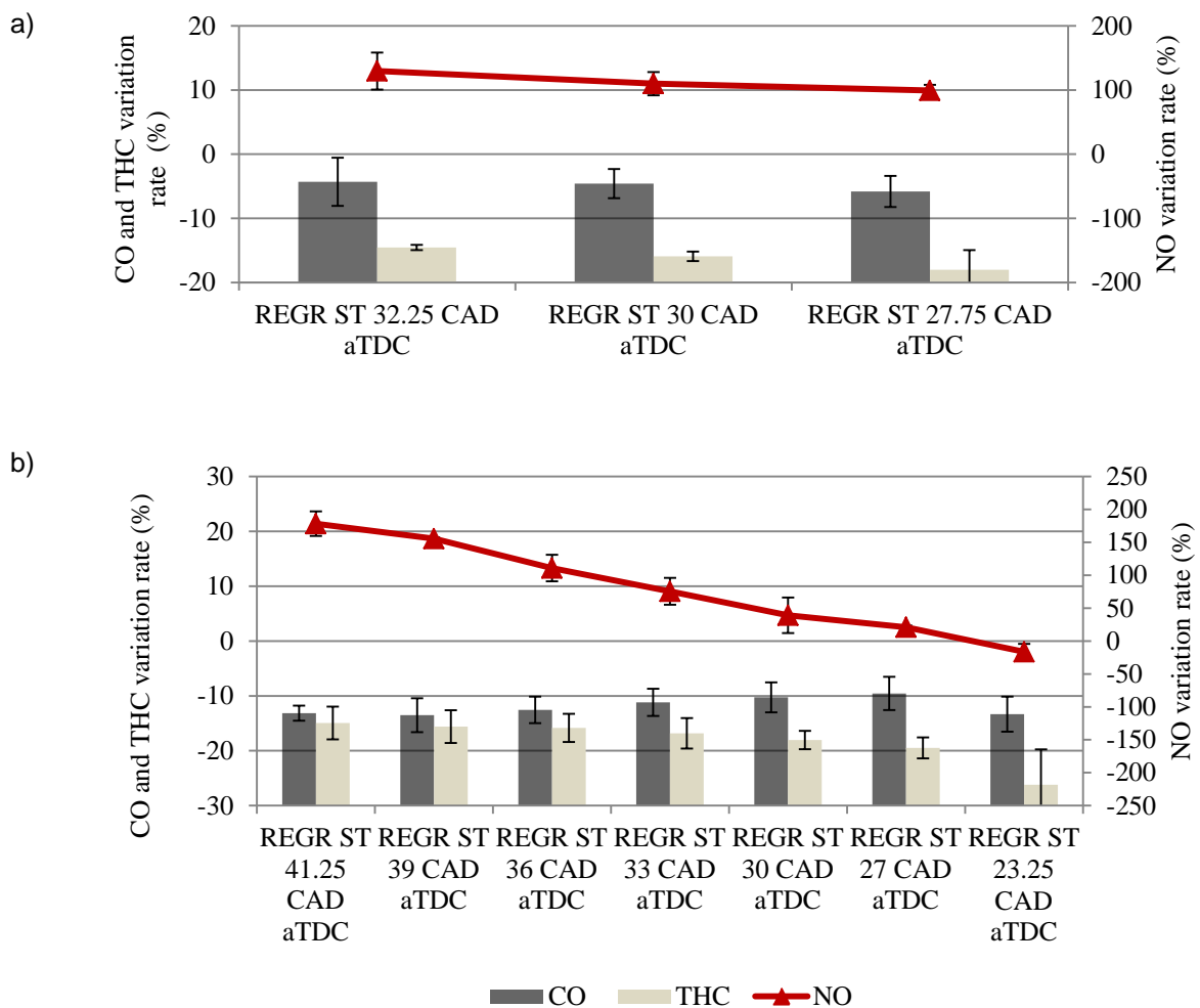
Figure 6. Effect of spark timing on gaseous emissions under REGR conditions at a) 303 CAD bTDC and b) 335 CAD bTDC.
