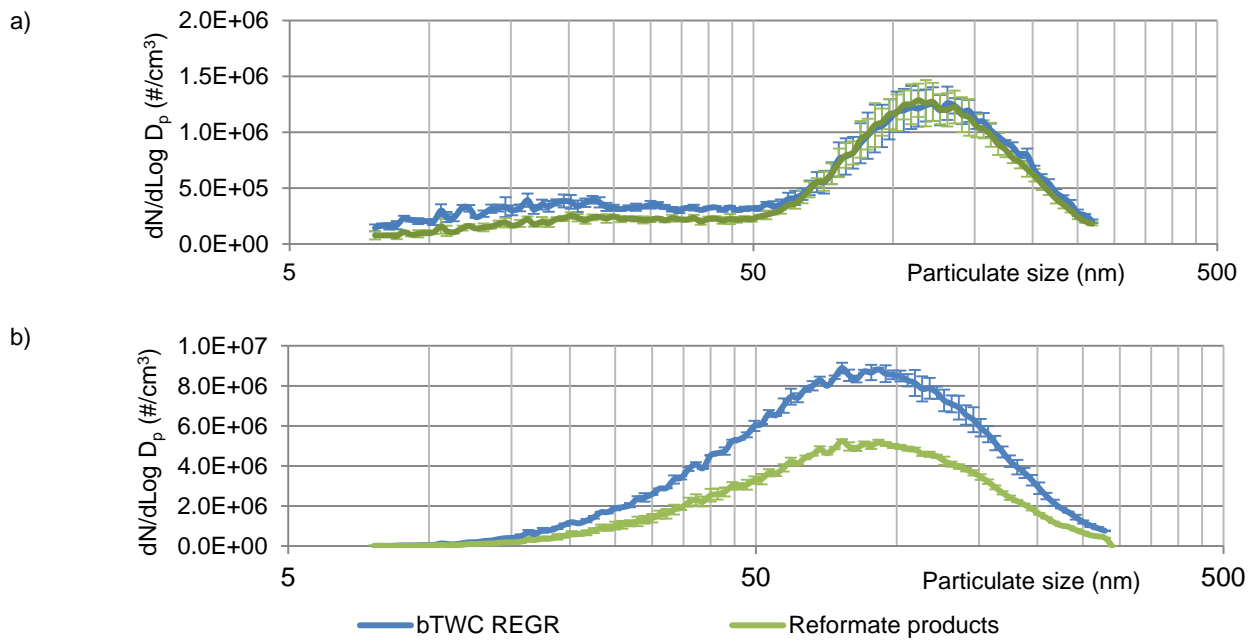
Figure 3. Effect of reformer on particulate size distributions at a) 303 CAD bTDC injection timing and b) 335 CAD bTDC injection timing.
