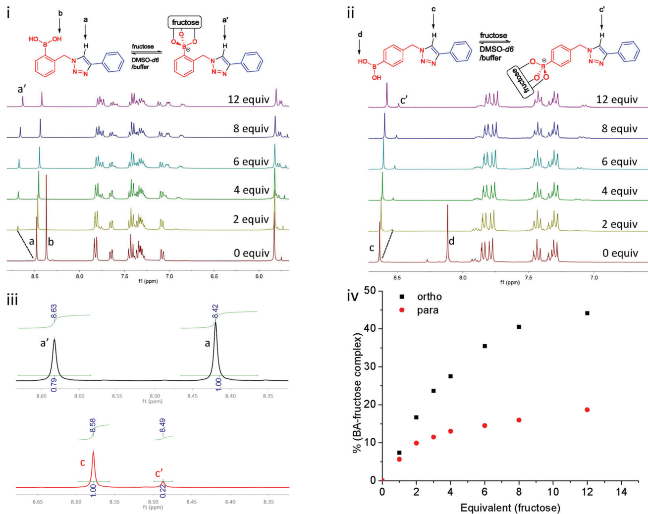
Fig. 4 (i) ^1\text{H} NMR titration of 1a with D-fructose in \text{DMSO-}d_6 and phosphate buffer solution (pD 8.21); (ii) ^1\text{H} NMR titration of 1c with D-fructose in \text{DMSO-}d_6 and phosphate buffer solution (pD 8.21), ^1\text{H} NMR drift slightly ( <0.1 ppm) due to the change of solvent composition during titration; (iii) integration of triazolyl protons for compound 1a (up) and 1c (bottom); (iv) the equivalent of fructose plotting against the percentage of BA-fructose complex in the system.
