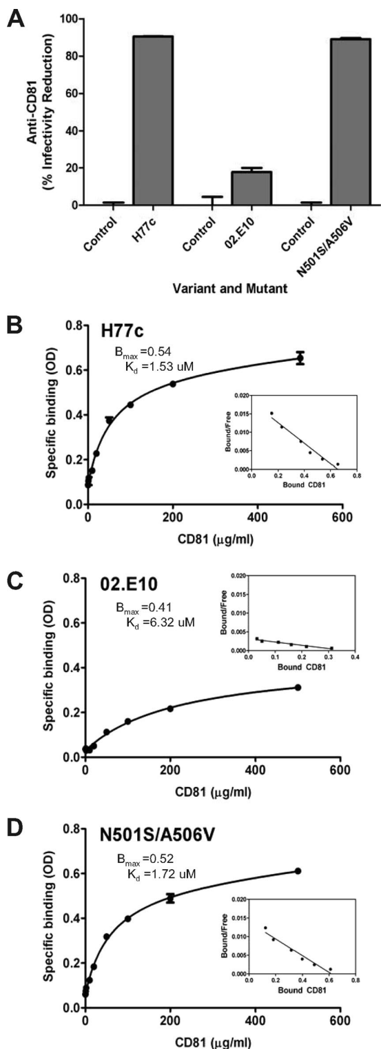
FIG. 3. Substitutions S501N/V506A in the context of the 02.E10 variant compromise binding of HCVpp to CD81. (A) Blocking of HCVpp infectivity by anti-CD81. Huh7.5 cells were preincubated with 5 \mu\text{g/ml} of anti-CD81 prior to infection with HCVpp bearing H77c, 02.E10, and 02.E10-N501S/A506V E2 envelope proteins. The control for each variant was without anti-CD81. The results are expressed as percentages of neutralization relative to the level for a no-antibody control for each variant or mutant, as measured by luciferase activity. N501S/A506V 02.E10 envelope protein to CD81 by ELISA. The bind-
