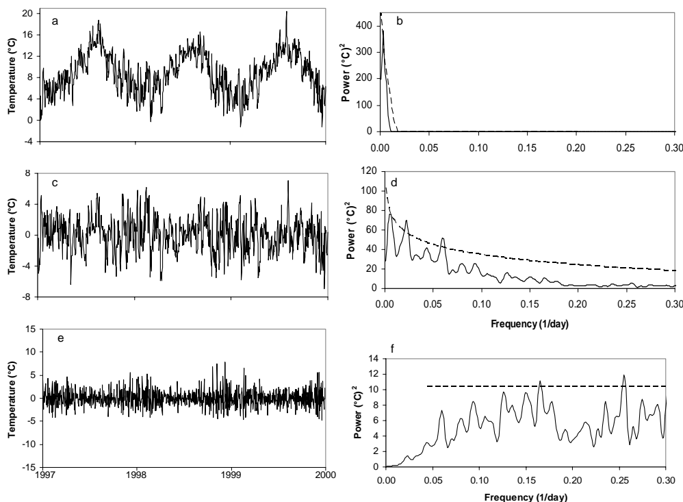
Figure 3. Illustration of some properties of time series using three years of daily temperature data from Stornoway, western Scotland as an example. The power spectra (b, d, f) illustrate the variation of the square of the temperature (power) with frequency of variation. Spectral analysis was performed with SPECTRUM software (Schulz and Statterger, 1997). Dashed lines in power spectra denote 95% confidence limit of significant spectral power (using approximately eight Hanning windows depending on resolution and length of series). a. raw data with a modelled annual cycle superimposed. b. most of the time series power is on the annual cycle (peak frequency 1/365). c. signal remaining when the annual cycle, modelled by a sine wave, is removed. Autocorrelation is still present, and can be attributed to the occurrence of synoptic weather conditions. d. Autocorrelated features show much low-frequency power (red noise pattern with some peaks, especially at frequencies of <0.1 , i.e. >10 days, corresponding to blocking weather patterns). e. Removal of the autocorrelation ('pre-whitening') leaves residual noise. The noise has higher amplitude in the winter. The procedure used was such that each pre-whitened temperature value at time t(T_p)_t = T_t - T_{t-1} * \rho_1 where T_t is the unwhitened value and \rho_1 is the coefficient of autocorrelation of the series with itself at a lag of one value. f. The remaining power spectrum has the characteristics of white noise. An effect of pre-processing is to enhance the significance level of very minor features of the raw data.
