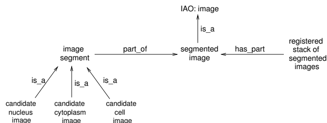
Figure 3. The ontology of Level 2. Image segments correspond to what we informally refer to as regions.
