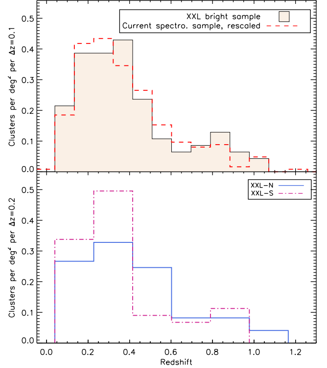
Fig. 4. Redshift distribution of the bright XXL cluster sample. Top: The bright sample compared with the distribution of 267 spectroscopically confirmed XXL clusters (to date). The latter has been rescaled to the same total number. Bottom: North/south fields separately (the bin width was doubled to obtain a shot noise comparable to that of the complete histogram).
