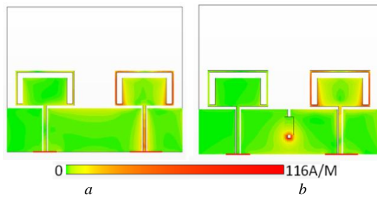
Fig.5 Current distribution
