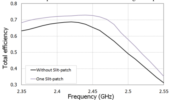
Fig.6 Total efficiency
