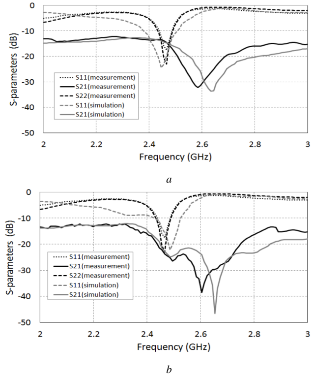
Fig. 2 Simulated and measured S-parameters a Two-element array (with a uniform ground plane) b A miniaturized slit-patch structure is inserted in the ground plane
