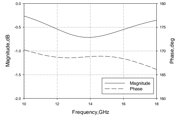
Fig. 3. Reflection magnitude and phase at PRS 1 .
