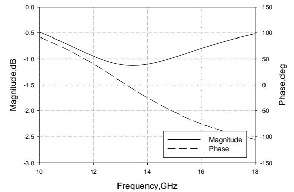
Fig. 4. Reflection magnitude and phase at AMC 2 .
