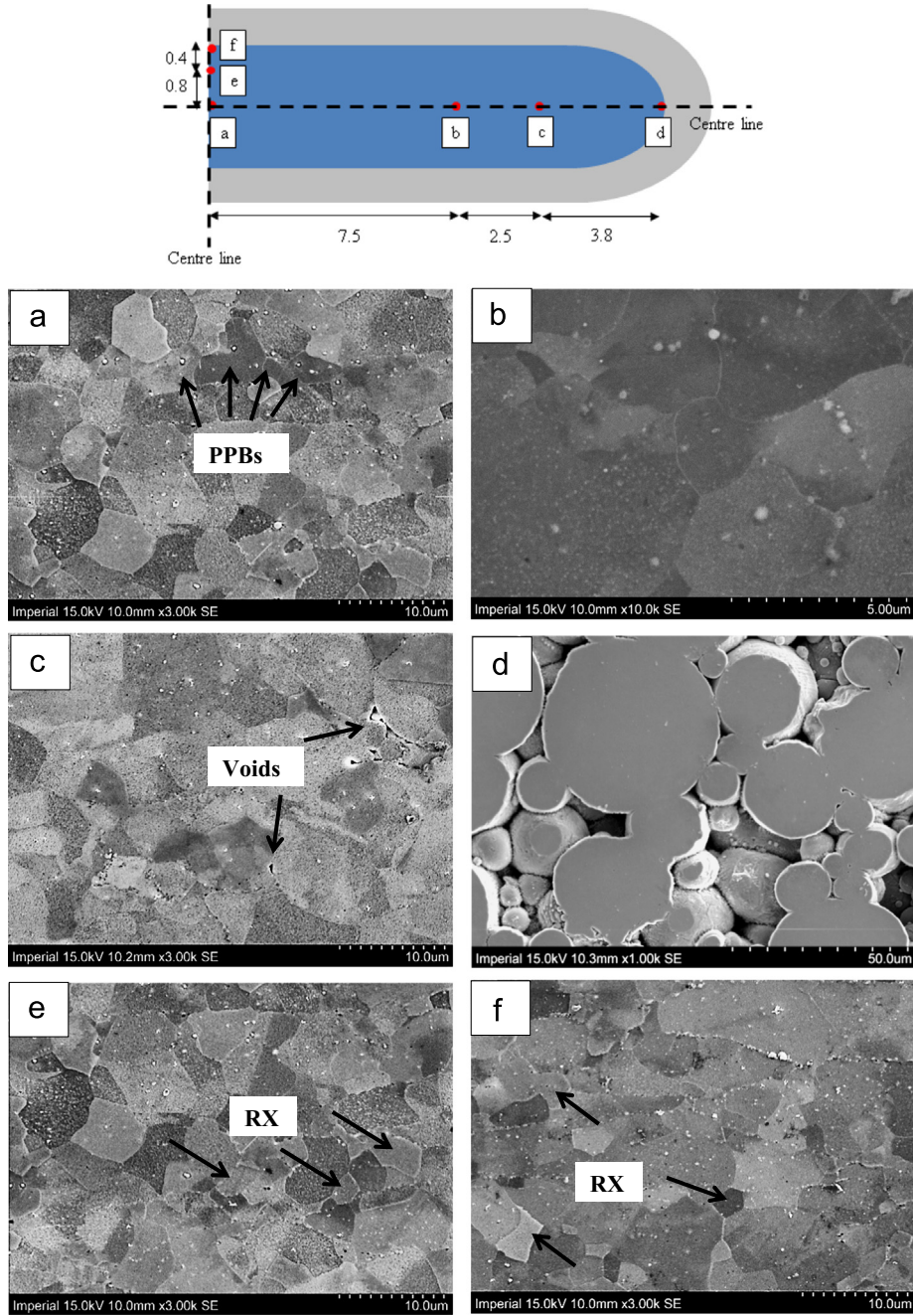
Fig. 3. SEM microstructure observation: typical microstructure at different locations (soaking temperature x1150 °C, soaking time 20 min, and forming speed 200 mm/s).
