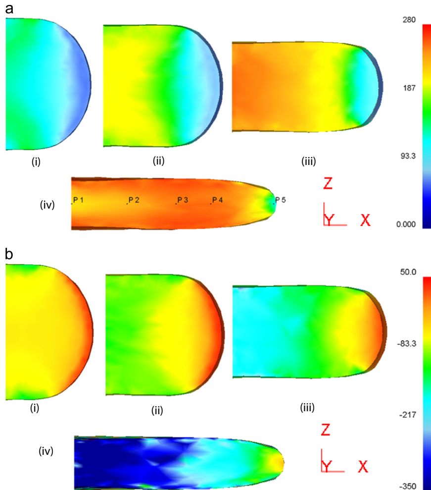
Fig. 8. Distribution of effective stress (MPa) (a) and mean stress (MPa) (b) at different times (MPa). t/t_f is (i) 25%, (ii) 50%, (iii) 75%, and (iv) 1 ( t_f is the final time).
