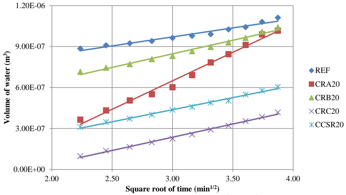
Fig. 10: Volume of water flowing into specimen with time
