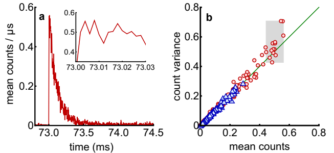
FIG. 3: Fluorescence measurements. (a) Fluorescence pulse, averaged over 250 drops. The exciting laser is pulsed on after the peak atomic density has passed through the cavity. At the start of the pulse, shown in detail in the inset, \langle N_{\text{eff}} \rangle = 1.24(5) . This is slightly larger than in Fig. 2 due to a higher atom number in the initial MOT. (b) Variance of fluorescence counts as a function of mean. Red circles are from the data used in (a), and blue triangles are from a set where the drive beam is pulsed on at a later time in the drop, with initial \langle N_{\text{eff}} \rangle = 0.50(2) . The green line is the photon shot-noise limit. The grey box corresponds to the inset in (a).
