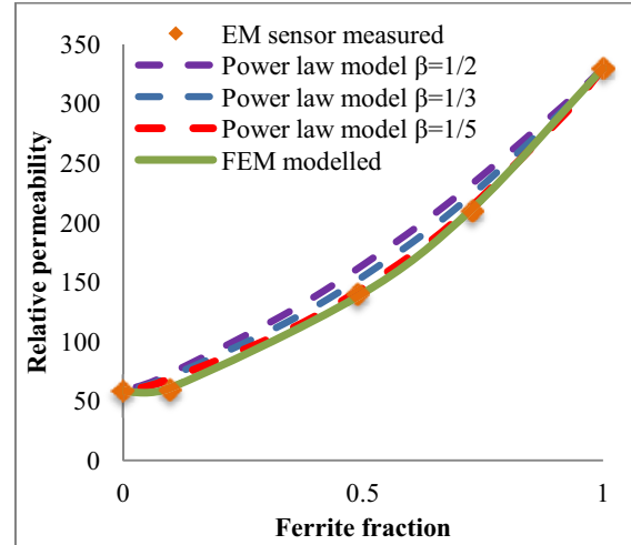
Figure 4. Relative permeability change with ferrite fraction, FEM modelled results were compared with the power-law model and the experimental fitted results.
