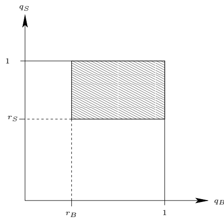
Figure 1. The region in which Ally-Ally is a Nash equilibrium when improved market performance is available.
