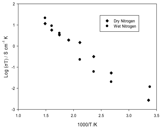
Fig. 12 Arrhenius plots of bulk conductivity for \text{Nd}_3\text{Zr}_2\text{Al}_{0.5}\text{Li}_{5.5}\text{O}_{12} in wet \text{N}_2 and dry \text{N}_2 .
