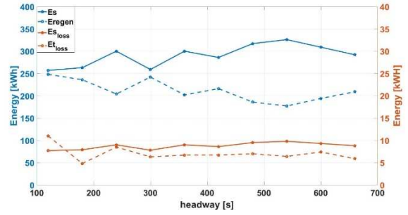
Fig.1- Energy evaluation for line A versus headways
