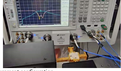
Fig. 9. Measurement configuration.
