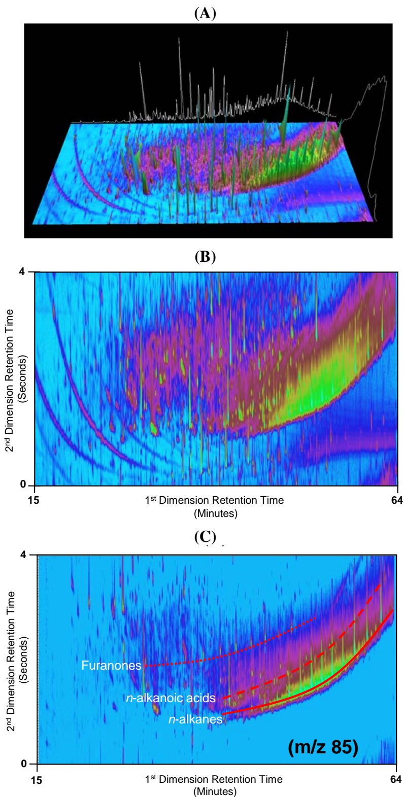
2 3 Figure 1. (A) Total ion current chromatogram of an urban aerosol sample (Birmingham, UK) examined by 4 GC×GC-TOFMS illustrating improved chromatographic resolution by GC×GC compared with GC/MS 5 (white line on background). (B) Contour plot of total ion current chromatogram of an urban aerosol sample 6 examined by GC×GC-TOFMS. Colours indicate the intensities of the response (green>yellow>pink). (C) 7 Example selected ion chromatogram ( m/z 85, n -alkane fragment). Red lines signify the ordered appearance 8 of compounds with similar physicochemical properties. Solid line – n -alkanes, dashed line – n -alkanoic 9 acids, dotted line – furanones with varying alkyl chain length. Sample taken 09-02-11. 10
