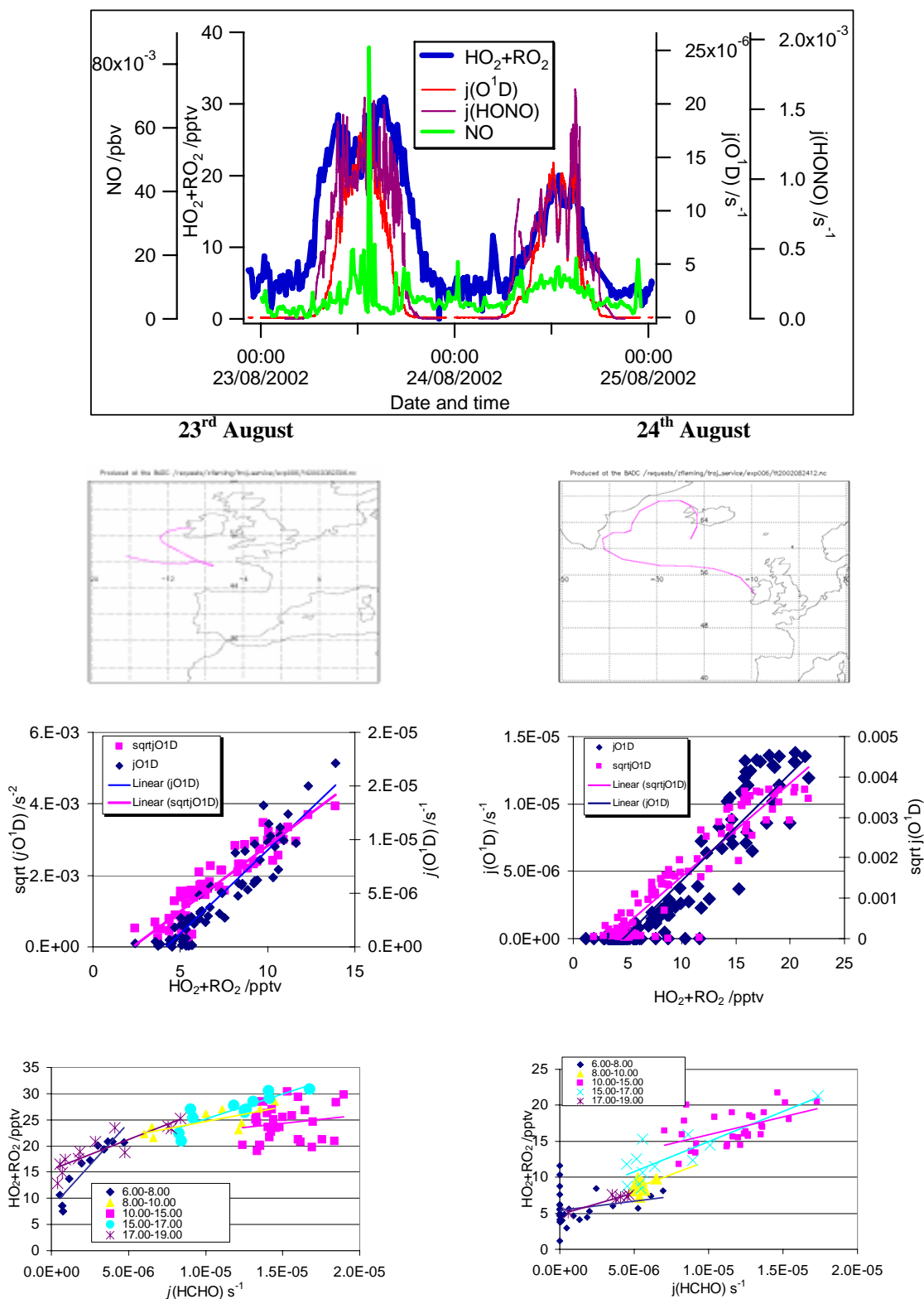
Fig. 5. Data for 23 and 24 August, \text{HO}_2+\sum\text{RO}_2 and j(\text{O}^1\text{D}) diurnal cycles and five-day back-trajectories. j(\text{O}^1\text{D}) and \sqrt{j(\text{O}^1\text{D})} vs. [\text{HO}_2+\sum\text{RO}_2] linear regressions and [\text{HO}_2+\sum\text{RO}_2] vs. j(\text{HCHO})_{\text{rad}} trends at different periods of the day are shown beneath the back-trajectories. The average concentrations/rates on 23 and 24 August where \text{NO}=6.3\pm 8.3, 7.3\pm 3.9 pptv, \text{HO}_2+\sum\text{RO}_2=14.7\pm 9.4, 8.3\pm 5.4 pptv, j(\text{O}^1\text{D})_{\text{day}}=7.3\times 10^{-6}\pm 5.7\times 10^{-6}, 5.5\times 10^{-6}\pm 4.8\times 10^{-6} \text{ s}^{-1} .
