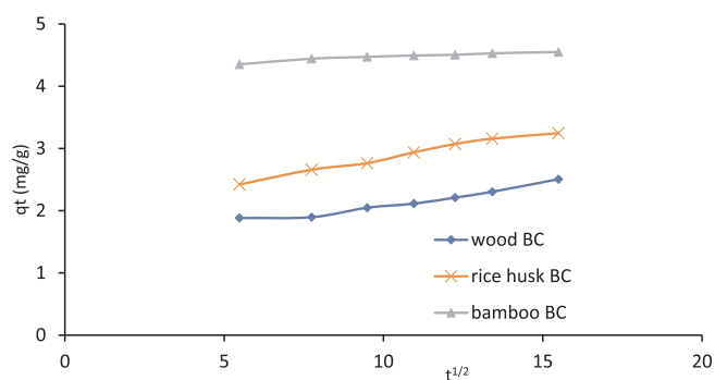
Fig. 4. Intraparticle diffusion plots for Zn^{2+} ions adsorbed onto the biochar. The value of q_t and the square root of t ( t^{1/2} ) were calculated using values from Fig. 3.
