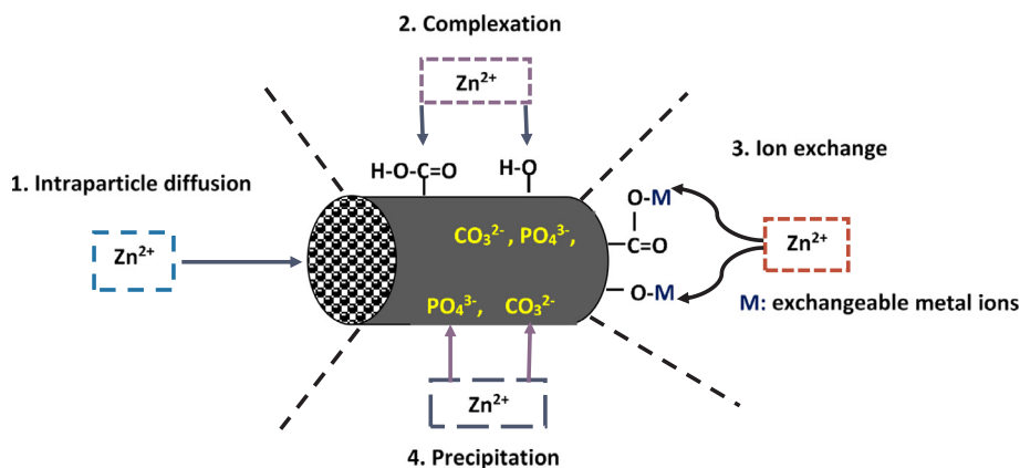
Fig. 5. Schematic of the mechanisms of Zn 2+ adsorption onto each of the three biochar.
