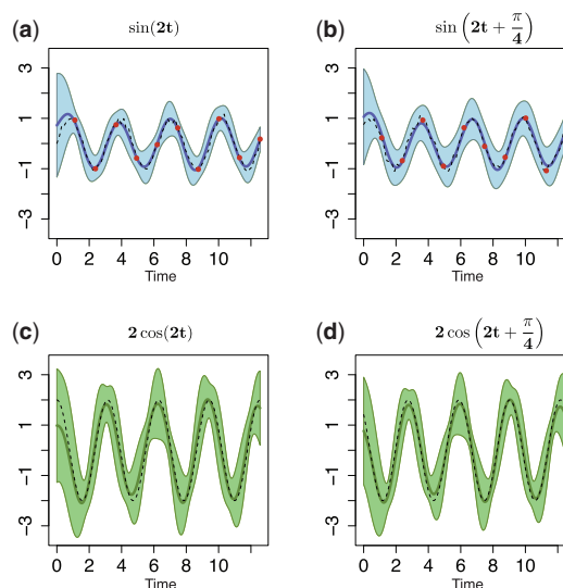
Fig. 1. Predictions with MGP model for two oscillating signals. (a and b) Dashed lines represent true behaviour of noiseless \sin(\cdot) trajectories; dots correspond to the noisy observations for both signals (data); solid lines are the mean behaviour of the MGPs model (predictions with original GPs); light areas correspond to two standard deviations at each prediction point. (c and d) Dashed lines represent true behaviour of noiseless \cos(\cdot) trajectories; solid lines show the mean behaviour of the MGPs model (predictions with derivative processes); light areas correspond to two standard deviations at each prediction point
