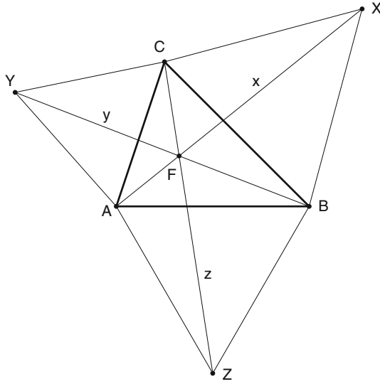
FIGURE 2. Fermat’s triangle theorem
