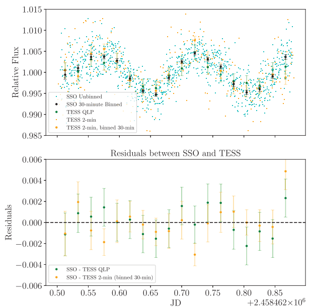
Figure 12. Top panel: SSO’s differential light curve compared to the light curves from TESS 2-min cadence data and MIT QLP 30-min cadence data for an M6V object ( J = 10.3 mag) on 2018 December 10. Bottom panel: the residuals between the TESS and SSO light curves.
