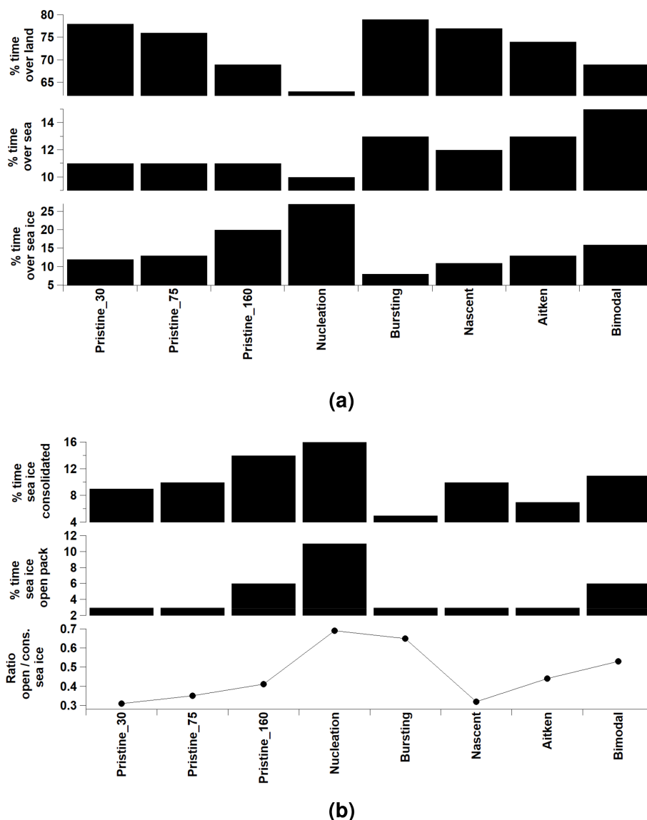
Figure 5. (a) Percentages of air masses over land, sea and sea ice for the eight k -mean aerosol categories and (b) percentages of consolidated and open-pack sea ice and the ratio of open-pack / consolidated sea ice.
