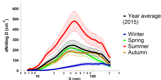
Figure 1. Seasonal mean aerosol size distribution measured by the SMPS at Halley VI over the year 2015. The error bars represent the standard deviation of the measurements from the mean value. D: diameter.
