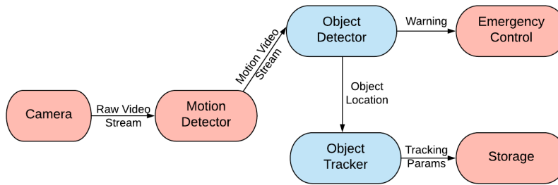
Figure 5: The flow diagram of iTransport application [34].
