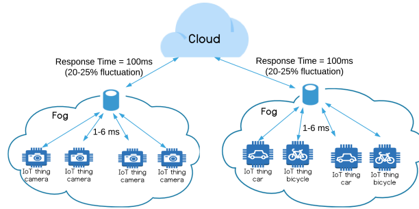
Figure 7: The Initial Experiment Configuration for iFogSim.
