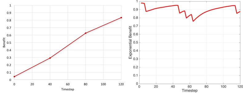
(a) Benefit for dao_6 (design-time) (b) Exponential Benefit for dao_6 (run-time)
