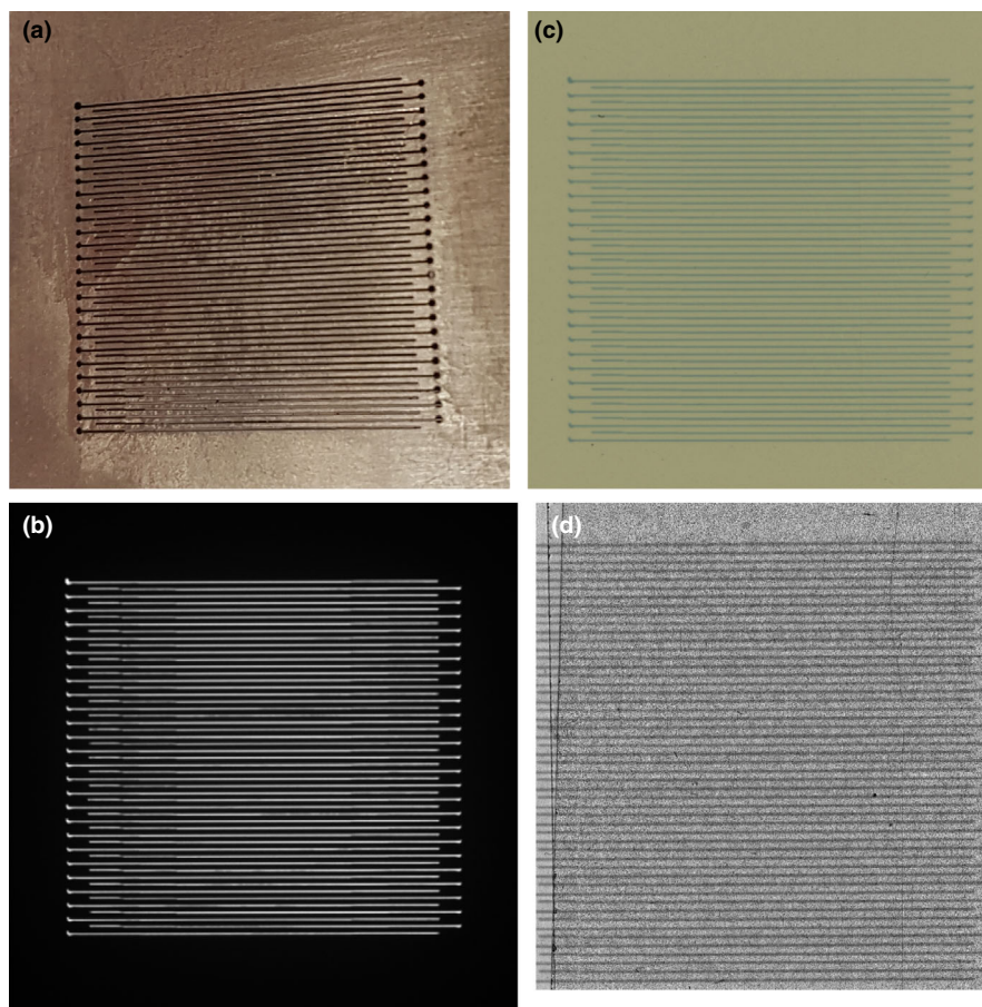
FIG. 2. (a) Photograph of microbeam collimator slits. (b) vM1212 detector image (cropped). (c) Scan of exposed EBT3 film using the Epson Expression 10000XL scanner ( 100\text{ }\mu\text{m} slit width). (d) Scan of exposed EBT3 film using Zeiss Axio Imager 2. [Color figure can be viewed at wileyonlinelibrary.com ]
