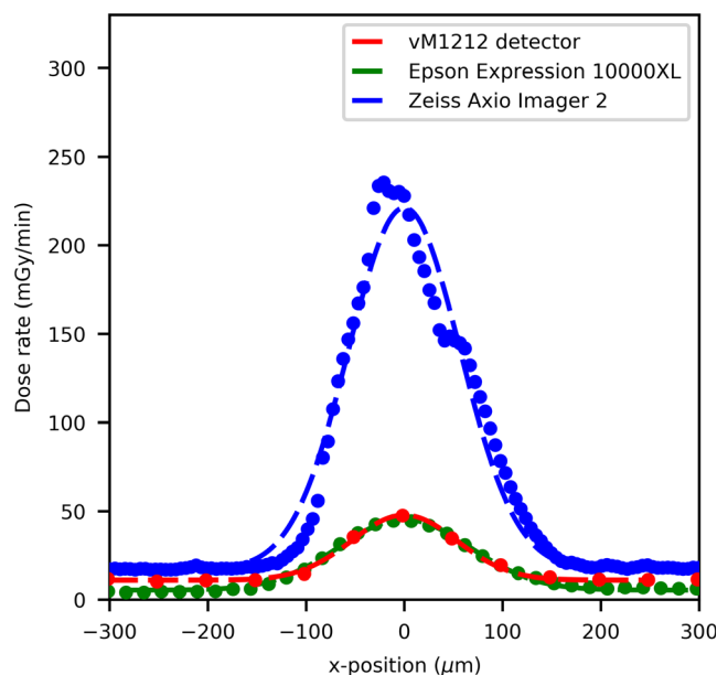
FIG. 7. 25 \mu\text{m} slit width peak profile comparison of the 26th central peak. [Color figure can be viewed at wileyonlinelibrary.com ]
